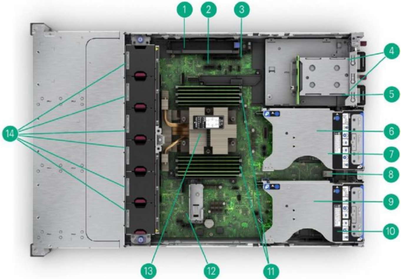
Internal View - 2SFF rear cage shown
